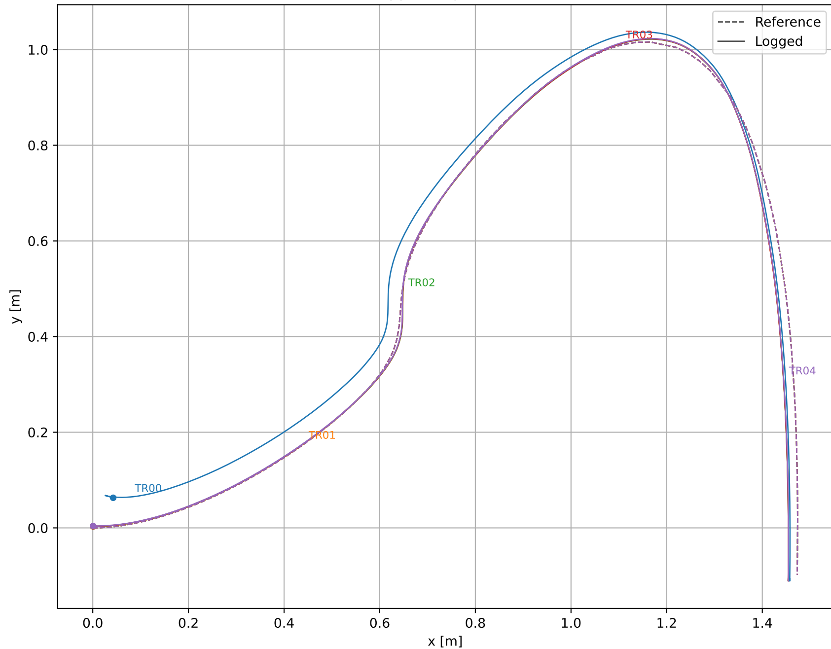
Logged Trajectories
